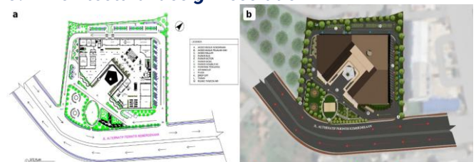
Figure 5. Site planning and circulation: (a) proposed site plan and landscape organization; (b) one-way vehicular loop, differentiated parking, pedestrian access, and planted perimeter. Source: author's design, 2026.
